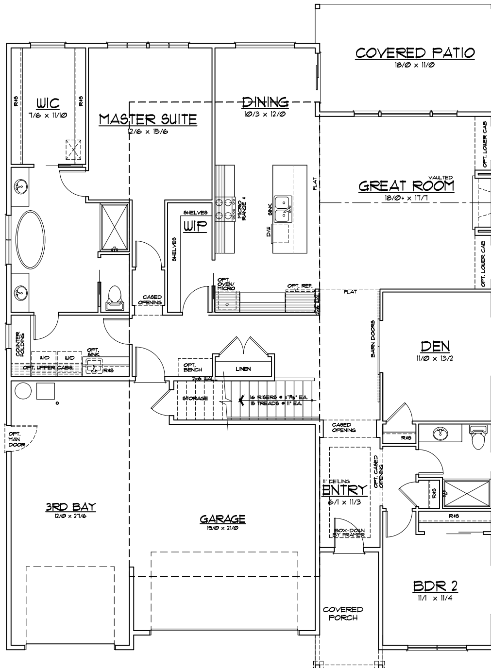
MAIN FLOOR PLAN - DESIGN
