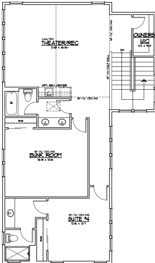
UPPER FLOOR LAYOUT - 1,238 SQ FT
