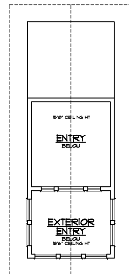
DORMER LAYOUT
